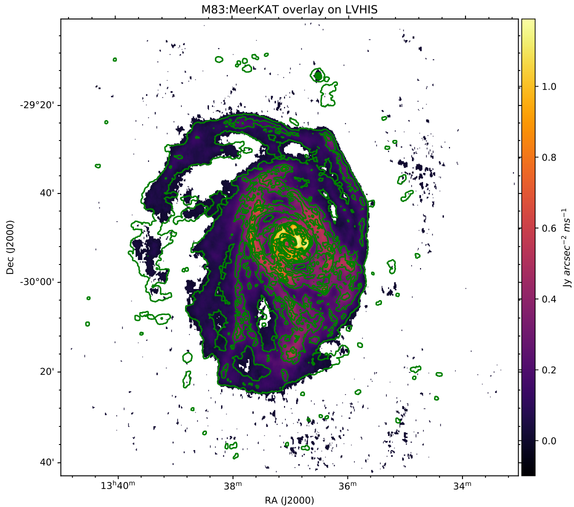
Figure 6: An overlay of the MeerKAT data (contours with levels) and the LVHIS 9-point mosaic of M83, done with ATCA, (beam = 85.8'' \times 60.8'' , natural weighting), observed 1998/9 Koribalski et al. (2018). The contours are the reduced MeerKAT data with contour levels of [0. 0.25 0.5 0.75 1. ] \text{Jy}/\text{arcsec}^2 \text{m.s}^{-1} and has a beam size of 24.88 by 23.56 arc-seconds.
